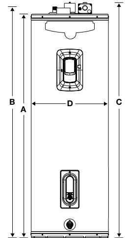
WATER CONNECTIONS ALL 3/4" N.P.T.
