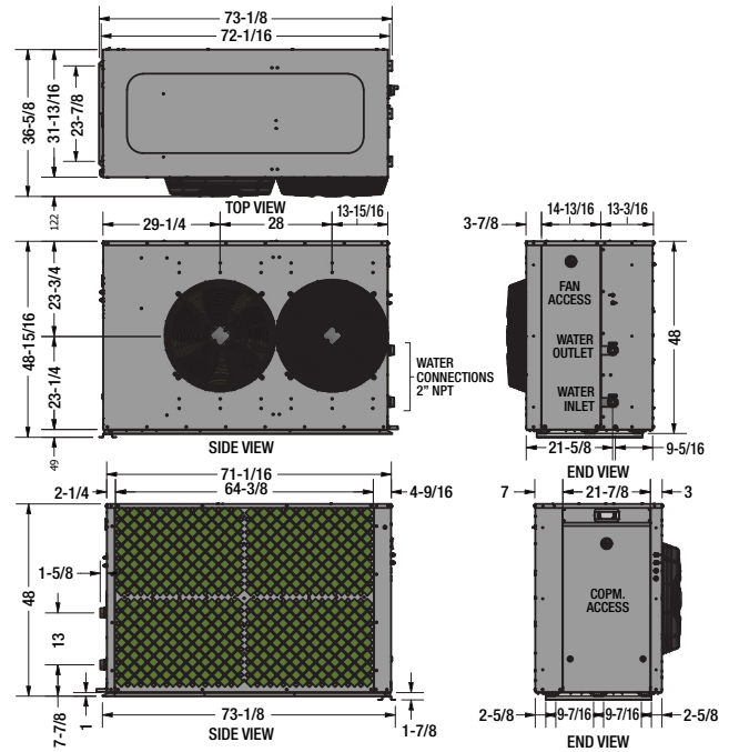
HPHD-135HNU-483 (Horizontal)
